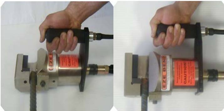
CAPACITY: #6 (3/4") 60-GRADE REBAR WEIGHT: 22 LBS.
