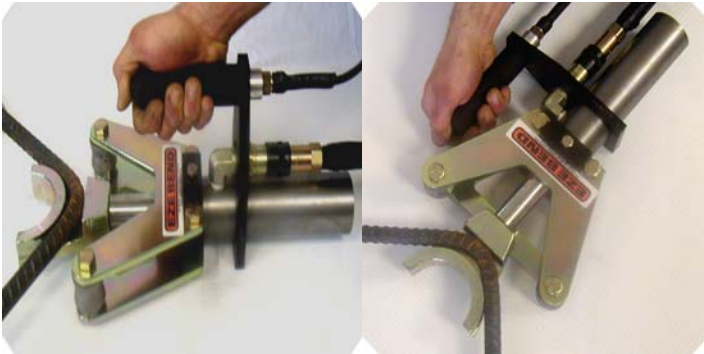
CAPACITY: #6 (3/4") 60-GRADE REBAR WEIGHT: 17 LBS.
