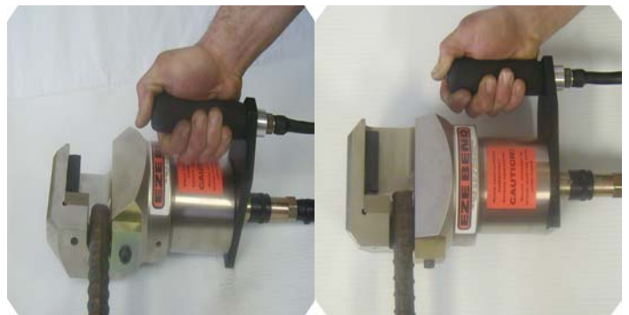
CAPACITY: #8 (1") 60-GRADE REBAR WEIGHT: 34 LBS.
