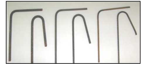
Tolman Tool Part # Open Cutter/Bender Bending Roller Dia.: 2.5"
